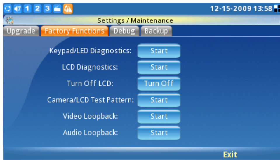
Figure 132: Factory Functions
