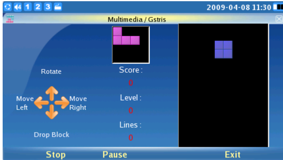
Figure 90: Gstris
