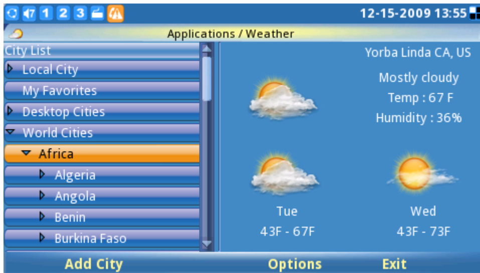
Figure 118: Weather Application
